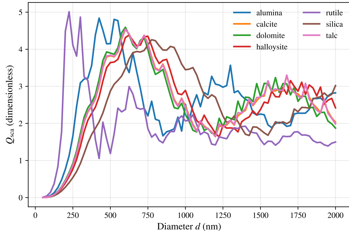
Sphere baseline optics at \lambda = 550 nm
