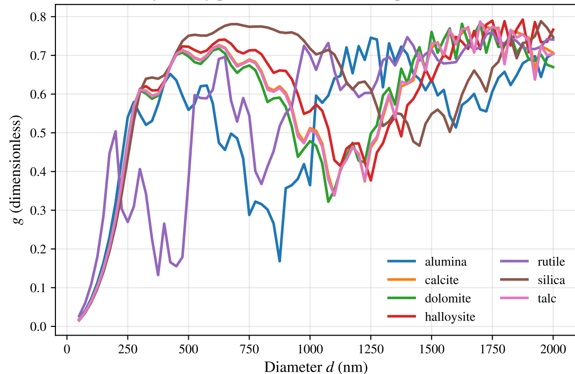
Asymmetry parameter at \lambda = 550 nm (sphere baseline)
