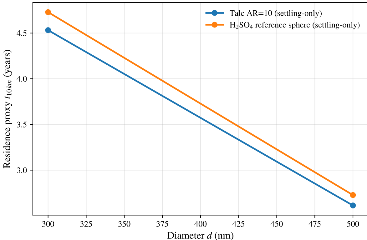
Settling-only residence proxy over 10 km at 20000 m (ISA)
