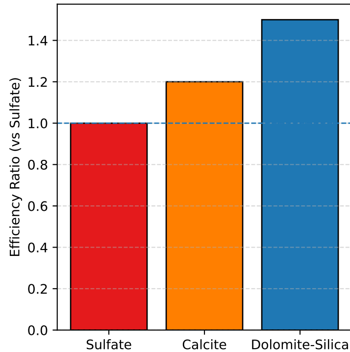
(a) Relative Optical Efficiency
